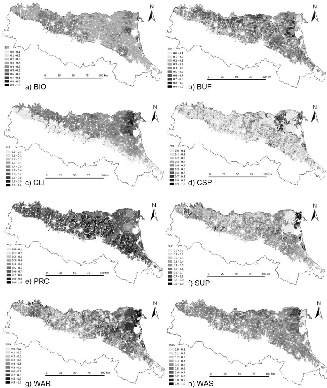
Fig. 3. Maps of soil functions. a) BIO: habitat for soil organisms; b) BUF: nutrient and pollutant retention and release; c) CLI: microclimate regulation; d) CSP: carbon sequestration potential; e) PRO: food provision; f) SUP: supporting human activities and infrastructures; g) WAR: runoff and flood control; h) WAS: water storage.
