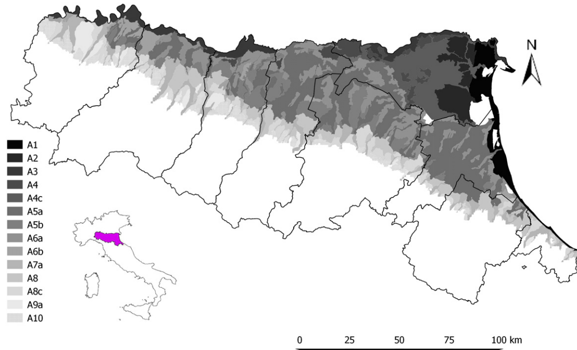
Fig. 1. Pedolandscape map of the Emilia-Romagna plain (Regione Emilia Romagna, 2012, mod.). A1: coarse textured soils of coastal plain; A2: Fine textured soils of the recently reclaimed areas of the Po river delta plain, with organic layers and peat; A3: Loamy textured soils of the meander plain of Po river; A4: Fine textured soils of the ancient depressions of Po river delta plain; A4c: Fine to loamy textured soils of the levee areas of the alluvial plain of the delta plain of Po river; A5a: Loamy textured soils of the levee areas of the Apennines recent alluvial plain; A5b: Loamy textured soils of the levee areas of the Apennines ancient alluvial plain; A6a: fine textured soils of the former depressions of the Apennines recent alluvial plain; A6b: fine textured soils of the former depressions of the Apennines ancient alluvial plain; A7a: Loamy textured soils of recent terraced areas of Apennines rivers, with presence of rock fragments; A8: Loamy textured soils of alluvial fans of Apennines, with rock fragments at variable depth; A8c: Fine to moderately fine textured soils of alluvial fans of Apennines, with strongly differentiated profile; A9a: Loamy skeletal soils of alluvial gravelly terraced fans, with highly differentiated profile; A10: Moderately fine to fine textured soils of the Apennine margin, with strongly differentiated profile.
